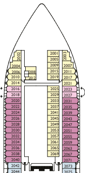
SARA DECK 2
